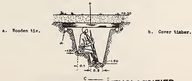
C-D Cross Section
