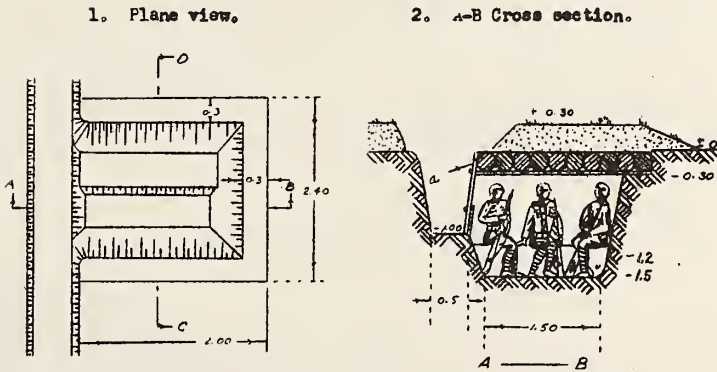
Illustration 101. Excavated type of light shelter.
